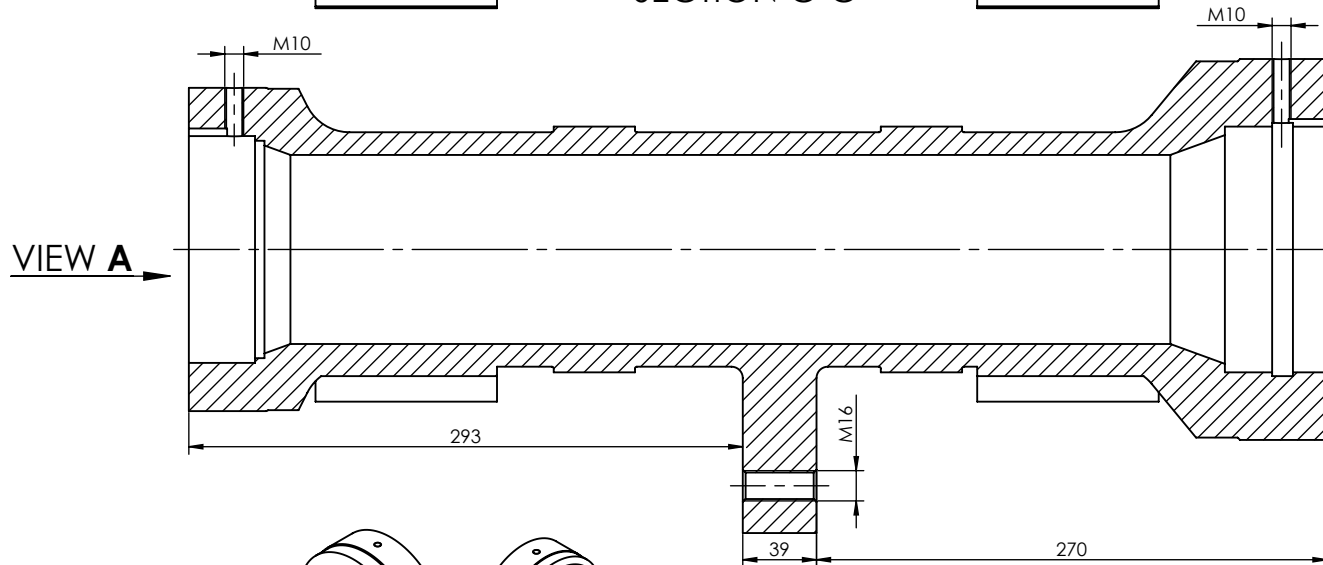
SECTION C-C
