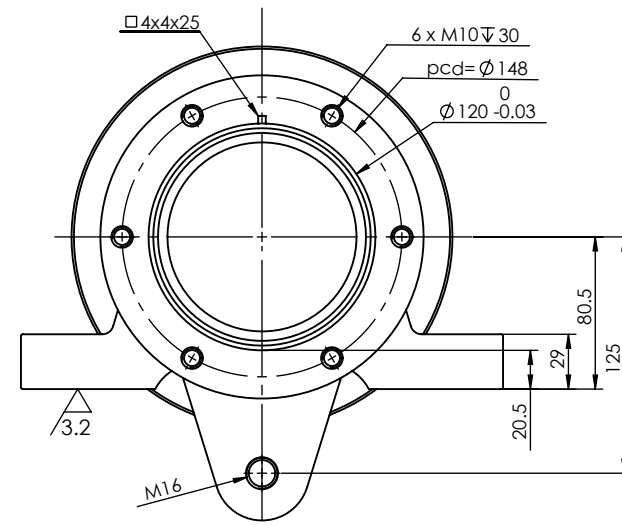
VIEW A
