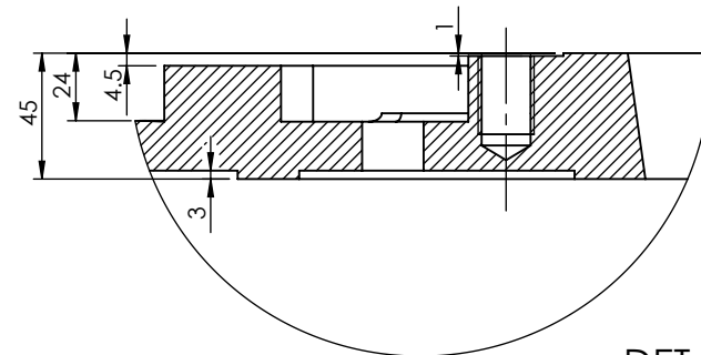
DETAIL B SCALE 1 : 3
